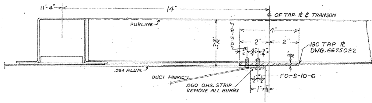
DETAIL "Z" HALF SCALE
