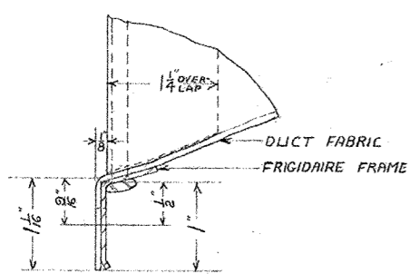
SECTION B-B FULL SCALE ROTATED LEFTWARD 90°
