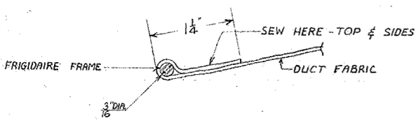
SECTION B-B FULL SCALE ROTATED LEFTWARD 90°
