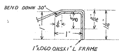
DETAIL "Y" FULL SCALE
