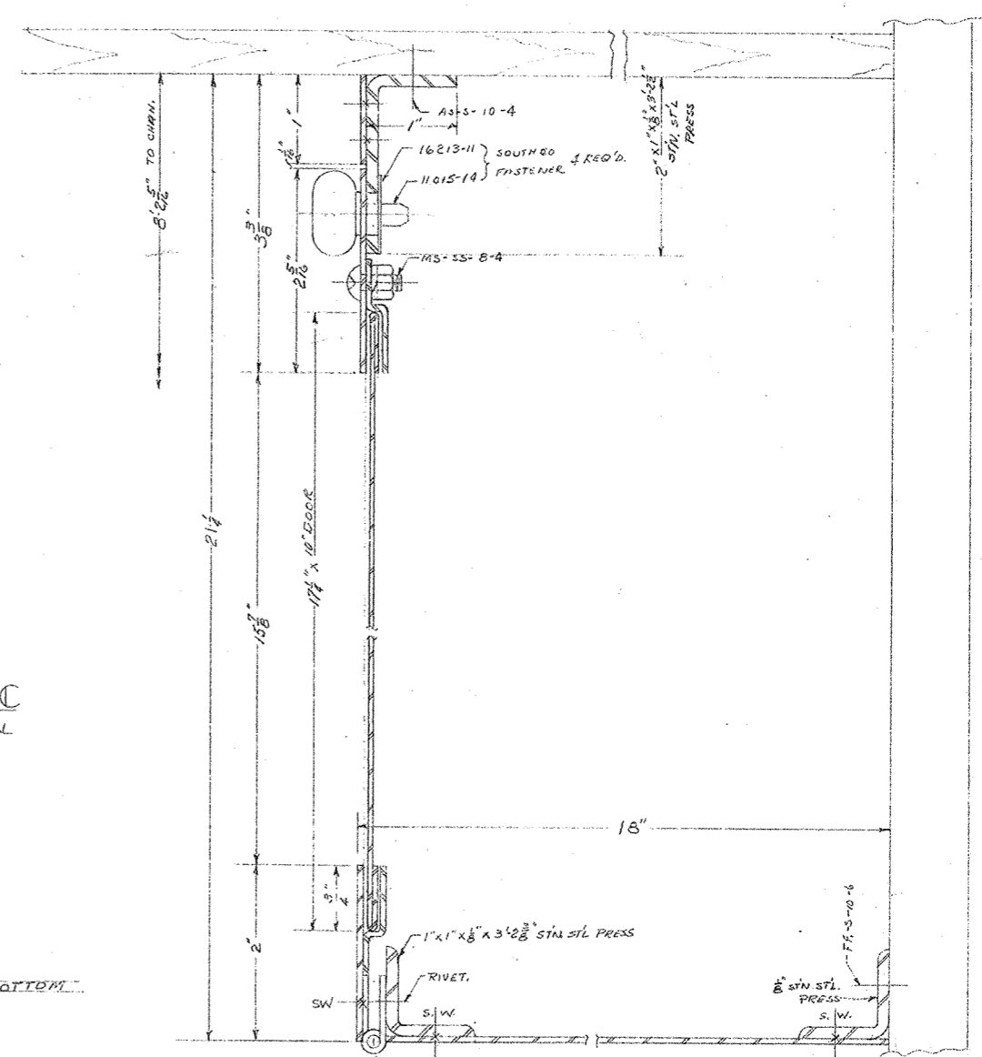
SS 7653 BRONSON SECTION B-B
