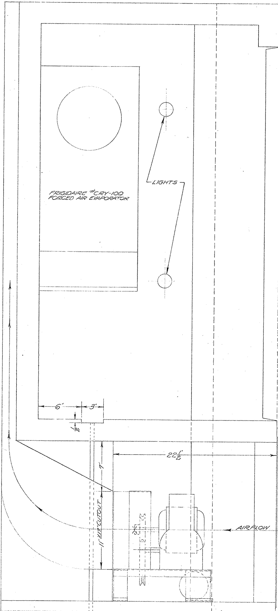
SECTION B-B
