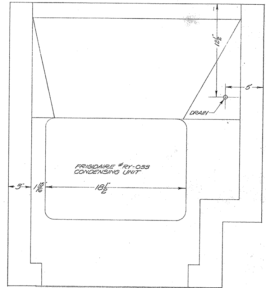
SECTION C-C
