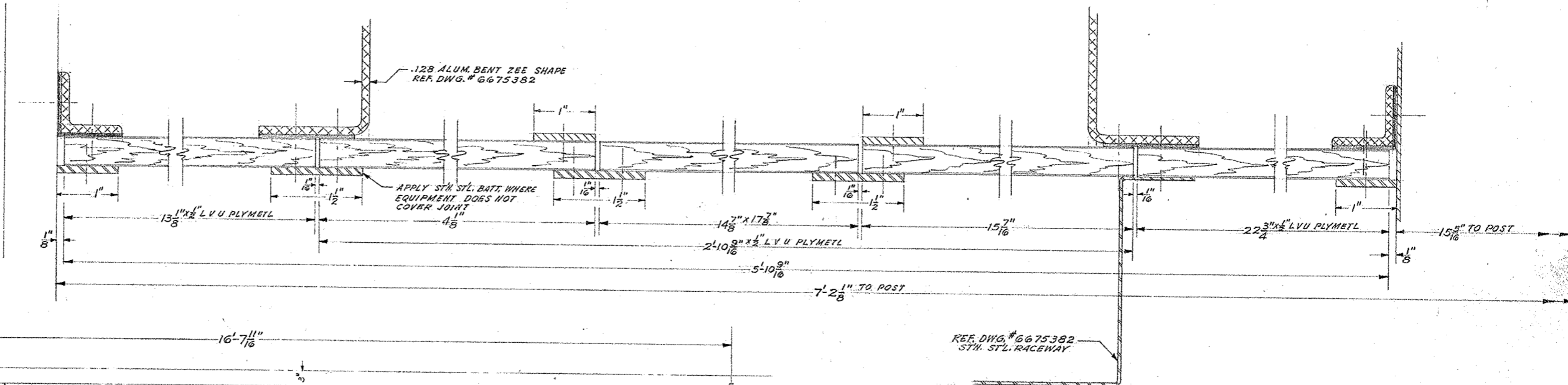
SECTION B-B
