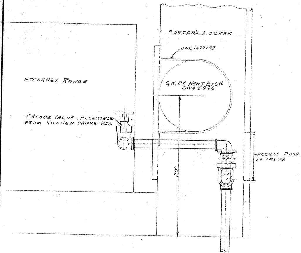
ELEVATION FACING RANGE
