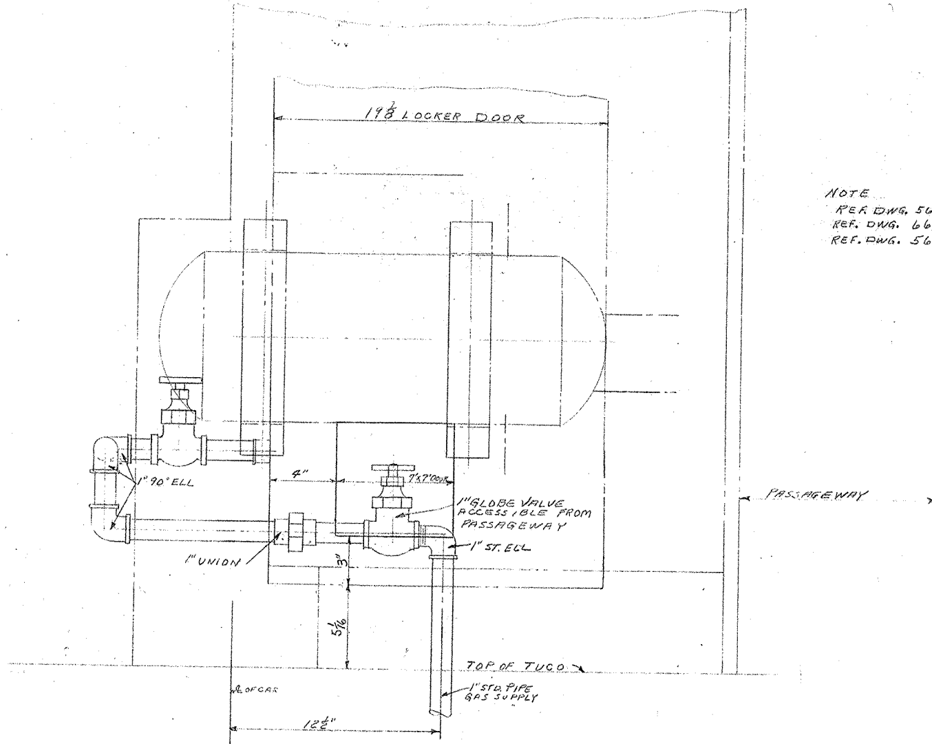
ELEVATION FACING PORTERS LOCKER
