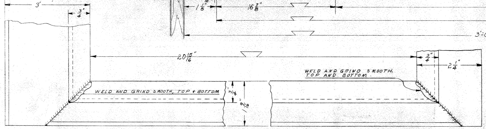
TYPICAL OF OPPOSITE SIDE DETAIL A
