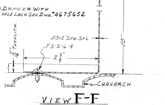
VIEW F-F
