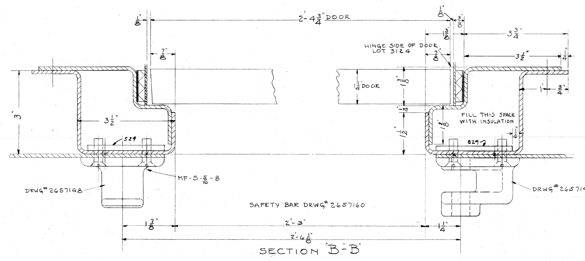
SECTION B-B
