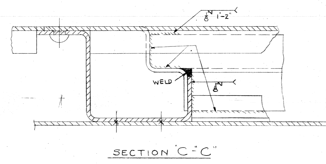
SECTION C-C
